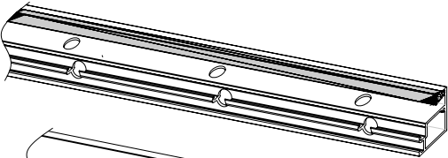
(A) (x2) 3,658mm (12ft) Profile with attached Gasket
