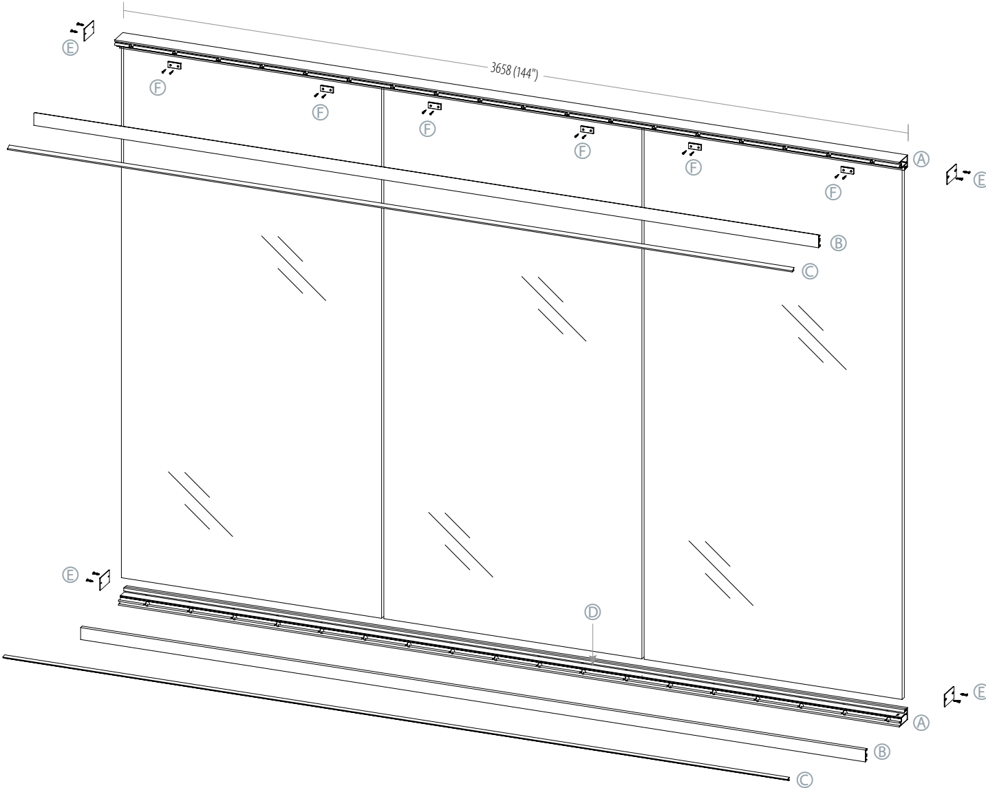
(F) (x6) Holder Plate (x12) Screw
