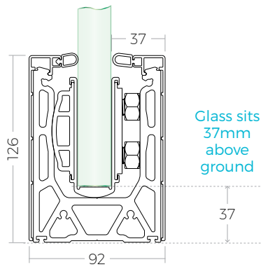
Top Mount Aluminum Cladding
