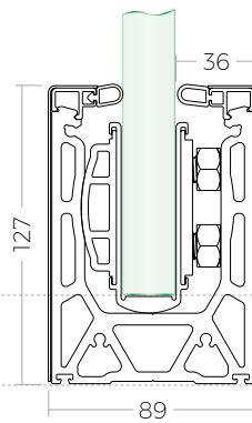
Top Mount Stainless Steel Cladding
