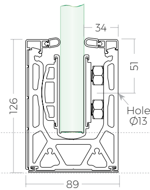
Side Mount Aluminum Cladding
