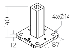
SSHPQR50B Blank Post
