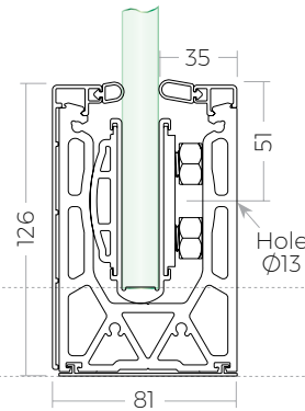
Side Mount Aluminum Cladding
