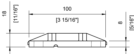
Plate Cover Scale: 1:2
