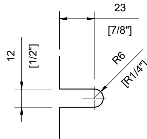
Glass Cut-out Scale: 1:2
