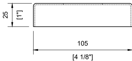
Plate Cover Scale: 1:2
