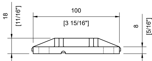
Plate Cover Scale: 1:2
