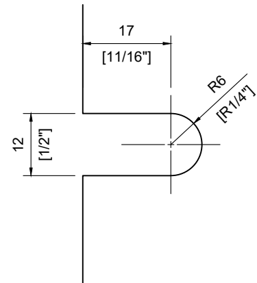
Glass Cut-out
