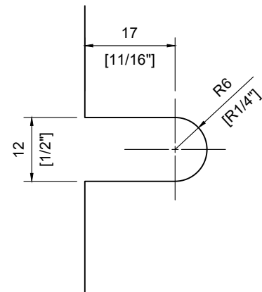
Glass Cut-out
