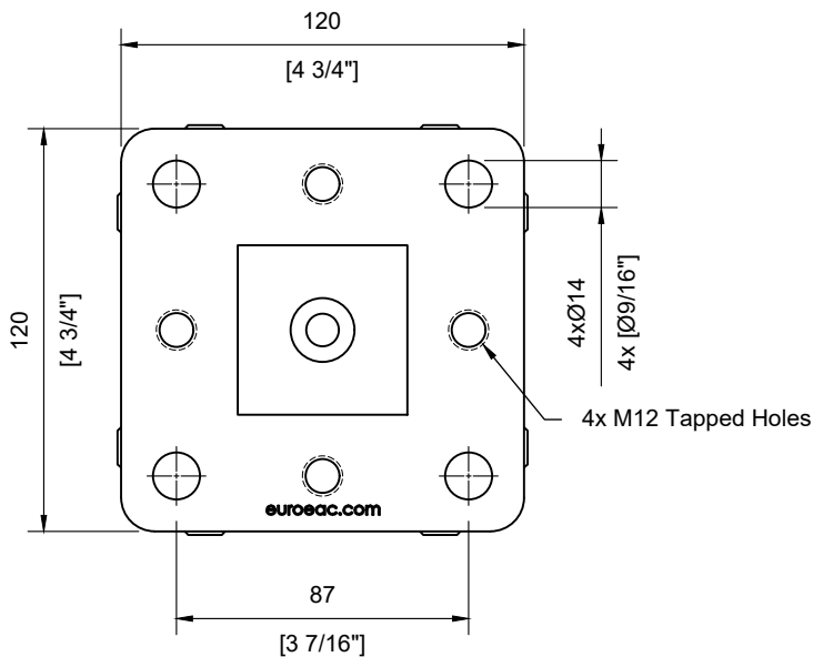
12mm [1/2"] Thick Base Plate Scale: 1:2
