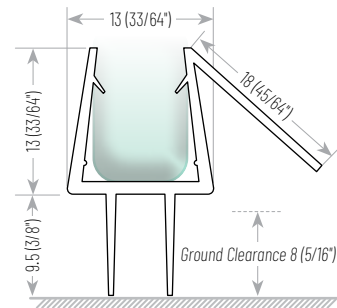
SSSFSSA • Glass to wall translucent gasket without adhesive strip • GLASS THICKNESS: 8 - 12mm • COMES IN: 300' Spools
