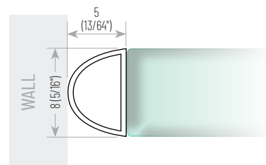
SSSFSSB • Glass to wall translucent gasket with adhesive strip • GLASS THICKNESS: 8 - 12mm • COMES IN: 300' Spools
