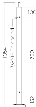
SSHPQR50C Corner Post
