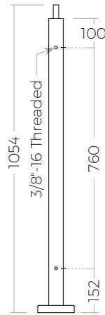
SSHPRND50C Corner Post
