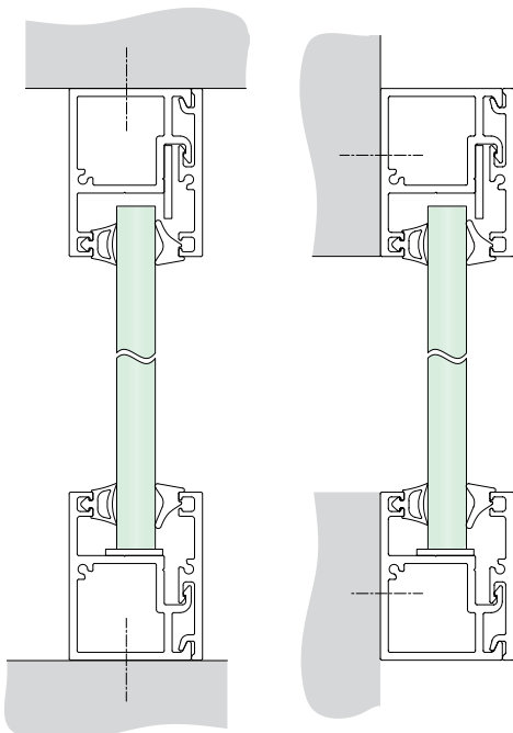
Top Mount
