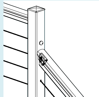
42" RAILINGS
