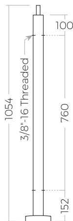
SSHPQR50L Line Post
