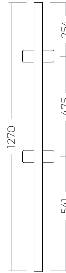
SSSPSQ40X42L Line Post 42"
