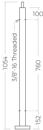
SSHPRND50L Line Post
