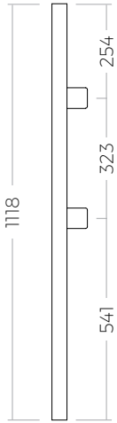
SSPSQ40X36E End Post 36"
