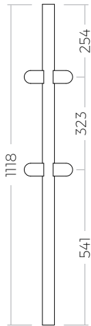
SSPG166X36L Line Post 36"
