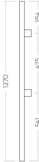
SSSPSQ40X42E End Post 42"
