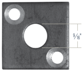
\frac{9}{16}'' PART# EPL5 W \frac{1}{8}'' H \frac{3}{32}''
