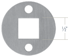
\frac{1}{2}'' PART# PSEPL2SS W \frac{111}{32}'' H \frac{1}{16}''
