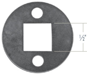
\frac{1}{2}'' PART# PSEPL2 W \frac{123}{64}'' H \frac{1}{16}''
