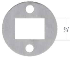
\frac{1}{2}'' \times \frac{3}{4}'' PART# PSEPL1SS W \frac{111}{32}'' H \frac{1}{16}''
