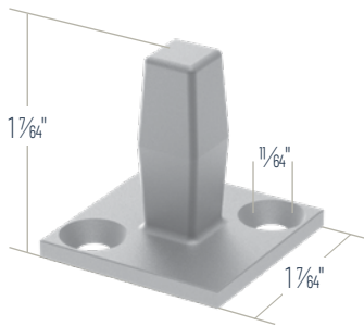
PART# EZTINSERT-A Use with 1/2" tubular balusters p 15-21
