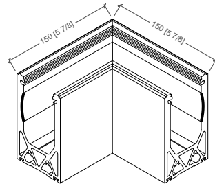
Outside Corner
