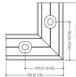
Inside Corner
