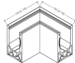
Inside Corner
