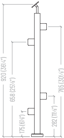
STAIR LINE - Front ④ SSPE36STLF
