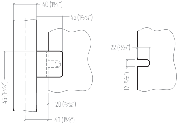
GLASS CLIP
