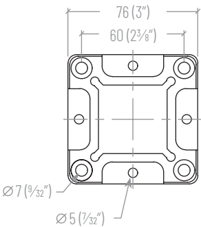
BASE PLATE
