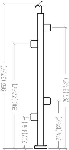
STAIR LINE - Middle ⑤ SSPE36STLM
