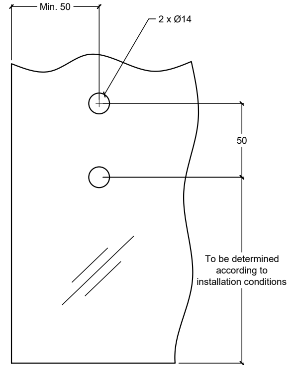
Glass cutting pattern
