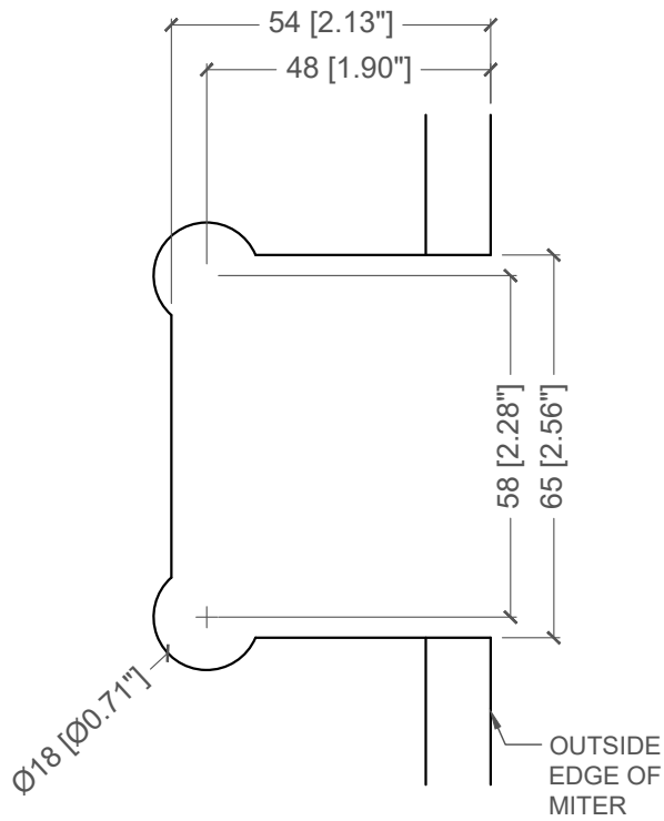
FIXED PANEL CUT-OUT
