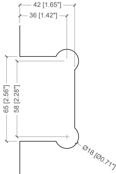
DOOR PANEL CUT-OUT
