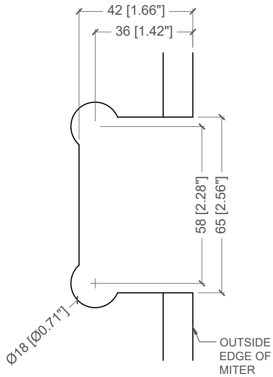
FIXED PANEL CUT-OUT
