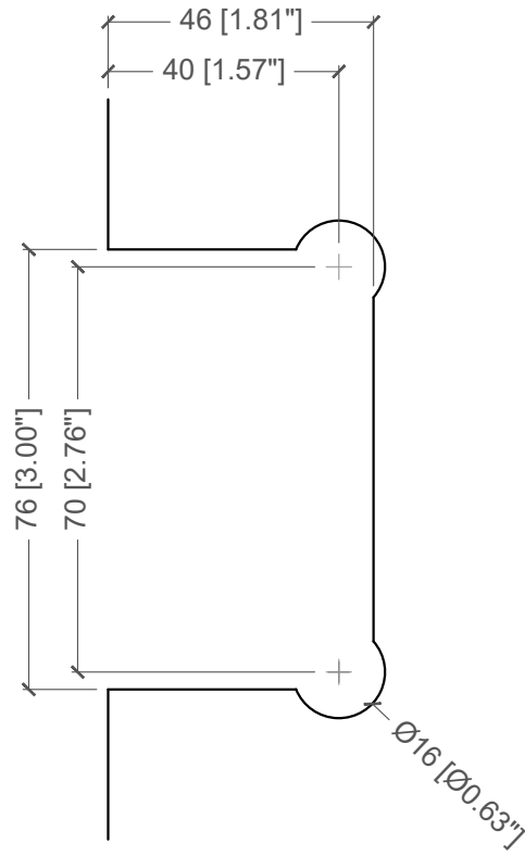
DOOR PANEL CUT-OUT
