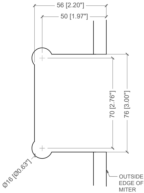
FIXED PANEL CUT-OUT
