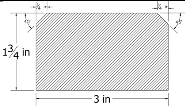
1 3/4" x 3" HANDRAIL - SQUARE/CHAMFER CORNERS 12 ft.
