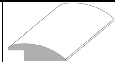
9/16" x 1 13/16" REDUCER - STANDARD
