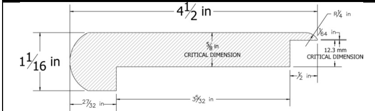
1 1/16" x 4 1/2" NOSING FOR LAMINATE
