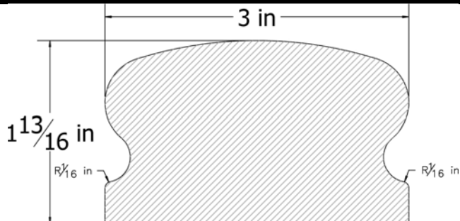
1 13/16" x 3" HANDRAIL 12 ft.
