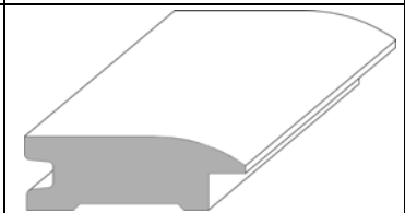
3/4" x 2 1/4" REDUCER - TILE
