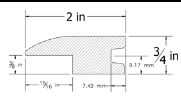
3/4" x 2" REDUCER - CARPET
