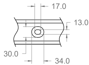
Hole Detail
