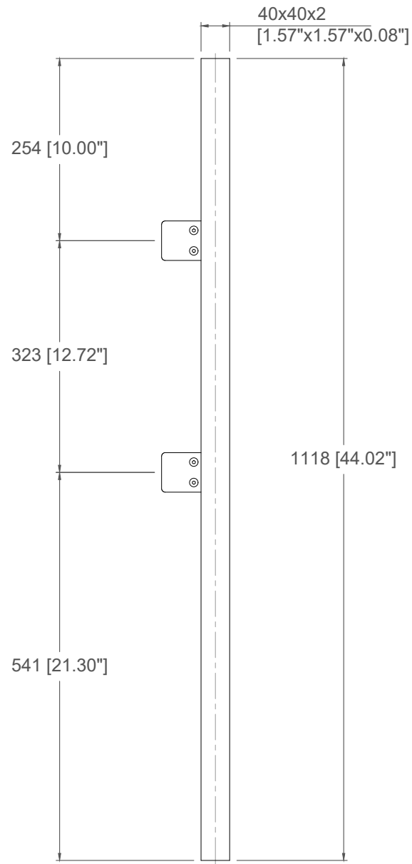
End Post SSPSQ40X36E
