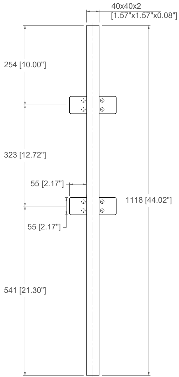
Line Post SSPSQ40X36L
