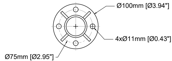
Base Plate
