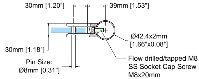
Typical Section
