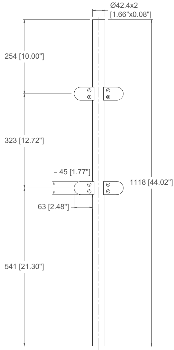
Line Post SSPG166X36L
