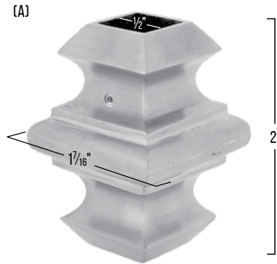
PART # 683SS12
