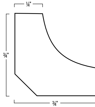
WCM120 - OAK WCM12HM - HARD MAPLE
