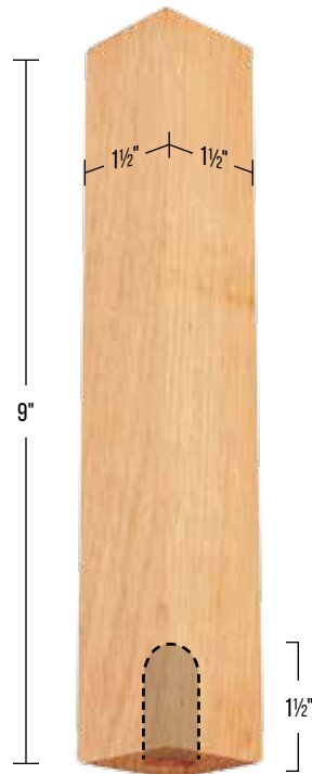
PART # WE9HM (HARD MAPLE) WE9O (OAK)
