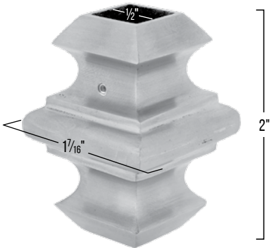
PART # 683SS12
