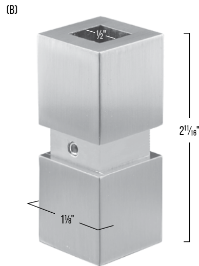
PART # PSMC112SS
